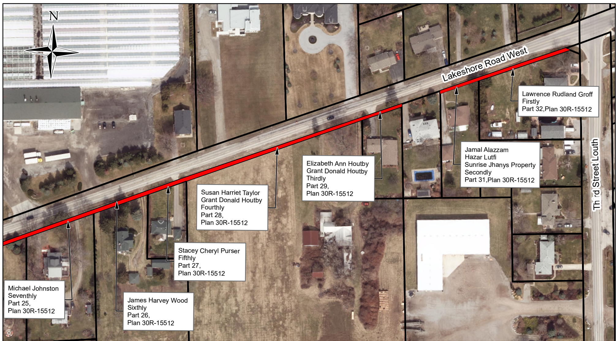
ILLUSTRATION SHOWING APPROXIMATE LOCATION OF ROAD WIDENINGS FROM VARIOUS OWNERS ALONG REGIONAL ROAD No.87 (LAKESHORE ROAD) WEST OF THIRD STREET LOUTH CITY OF ST. CATHARINES
